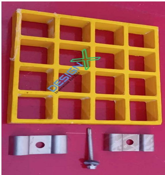
FRP-Walk Ways,25,30,38,50mm
